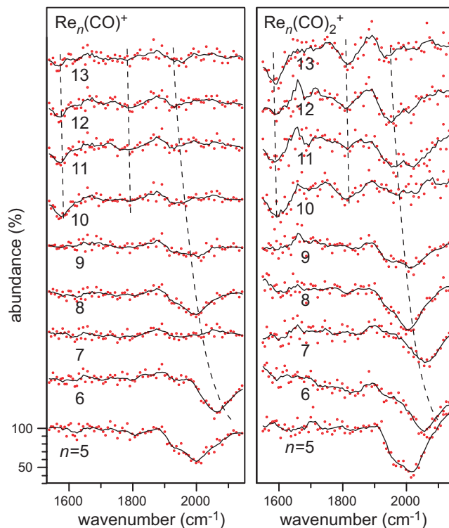
FIG. 3. IR-MPD spectra of one and two carbon monoxide molecules adsorbed to cationic \text{Re}_n^+ clusters ( n=5\text{--}14 ). The red dots are the actual data points, while the black line interconnects its adjacent three point average. The dashed vertical lines indicate the approximate position of the CO absorptions for this cluster size range.
