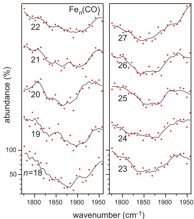
FIG. 1. IR-MPD spectra of a single carbon monoxide molecules adsorbed to neutral \text{Fe}_n clusters ( n=18\text{--}27 ). The red dots are the actual data points, while the black line interconnects its adjacent three point average.
