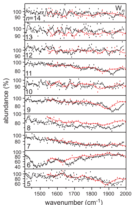
FIG. 4. IR-MPD spectra of ^{12}\text{CO} (black) and ^{13}\text{CO} (red) molecules adsorbed to neutral \text{W}_n clusters ( n=5-14 ). The dots are the actual data points, while the lines interconnect its adjacent three point average.
