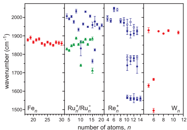
FIG. 5. A plot of the observed CO stretching frequency on metal clusters ( \text{M}_n ) vs cluster size n . From left to right, the first panel indicates the observed frequency on neutral iron clusters (red circles). The second panel indicates the observed frequency on cationic (blue squares) and anionic (green triangles) ruthenium clusters. The third panel indicates the observed frequency of one (solid blue squares) and two (open blue squares) CO molecules adsorbed on cationic rhenium clusters. The fourth panel indicates the observed frequency on neutral tungsten clusters (red circles). The peak positions are determined from a least-squares fit to a Gaussian line shape. The error bars indicate twice the standard deviation ( 1\sigma ) of the fits.
